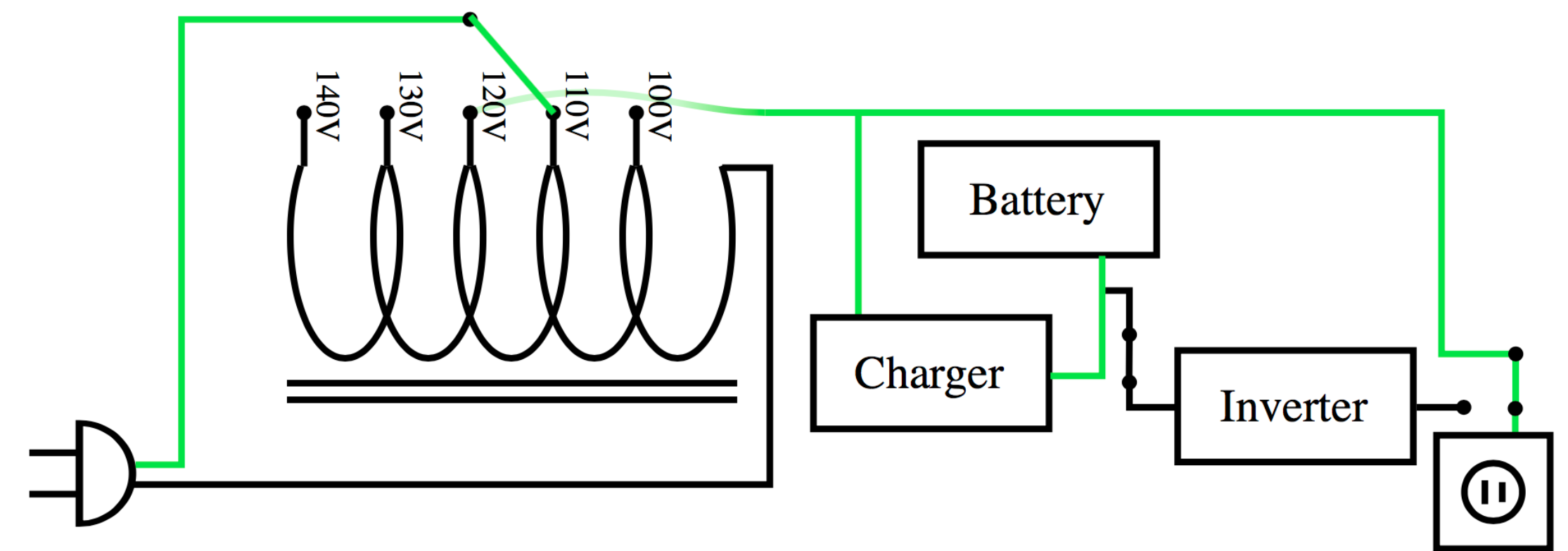
Small Undervoltage
