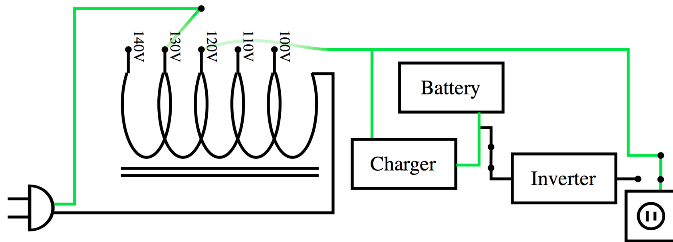
Small Overvoltage
